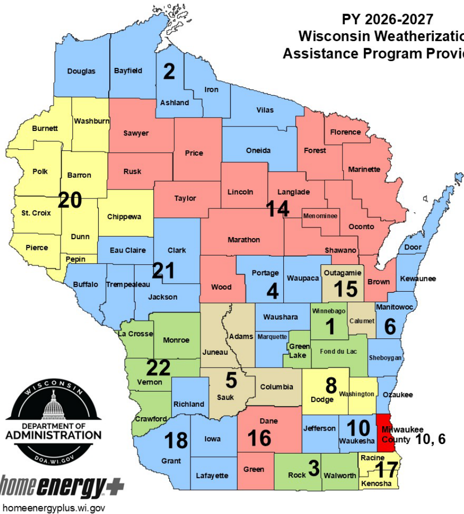
Weatherization Providers by Provider Number
