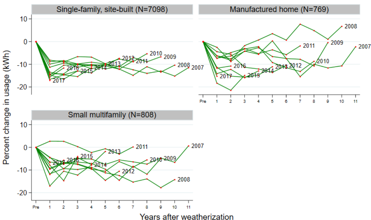
Figure 2. Percent change in electricity usage compared to pre-weatherization
