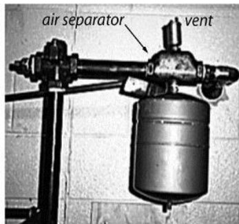
Expansion tank, air separator, and vent: Preventing excessive pressure and eliminating air from the systems are important for hydronic distribution systems.
