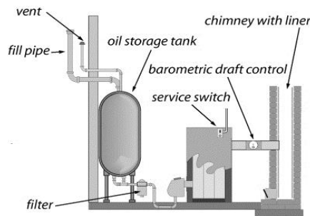
Oil heating system: Components of an oil heating system may need repair and cleaning during replacement of the furnace or boiler.
