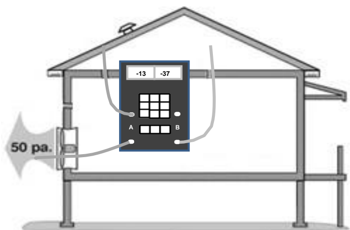
Attic-to-outdoors pressure: The left side of the gauge shows an attic WRT outside pressure of -13 pascals and the right side of the gauge shows a House WRT Attic pressure of -37 pascals. The two readings add up to -50 pascals to confirm House WRT Outside of 50 pascals.
