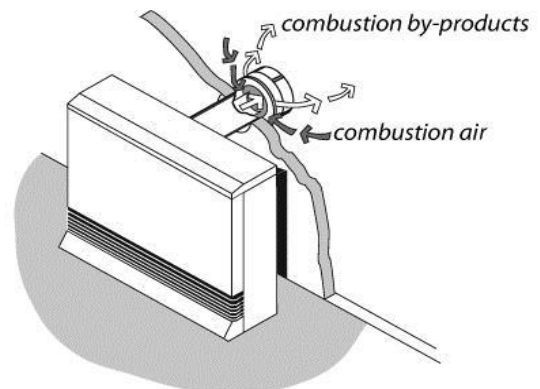
Sealed combustion space heater: A sealed combustion space heater draws combustion air in and exhausts combustion by-products through a concentric vent system using a draft fan.
