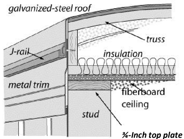
Bowstring roof details: Hundreds of thousands of older manufactured homes were constructed with these general construction details.
